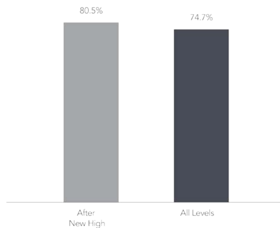
Exhibit 1. S&P Total Return Index Highs: 1926–2016 Percent of Months With Positive Return Over Next 12-Month Period
